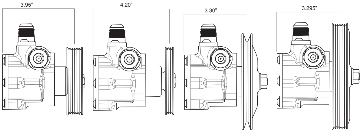
6-Groove Serpentine Pulley Pump Rotated 90° Not to Scale 3-Groove Serpentine Pulley Pump Rotated 90° Not to Scale GM Offset V-Belt Pulley Pump Rotated 90° Not to Scale 6-Groove LS Serpentine Pulley Pump Rotated 90° Not to Scale
