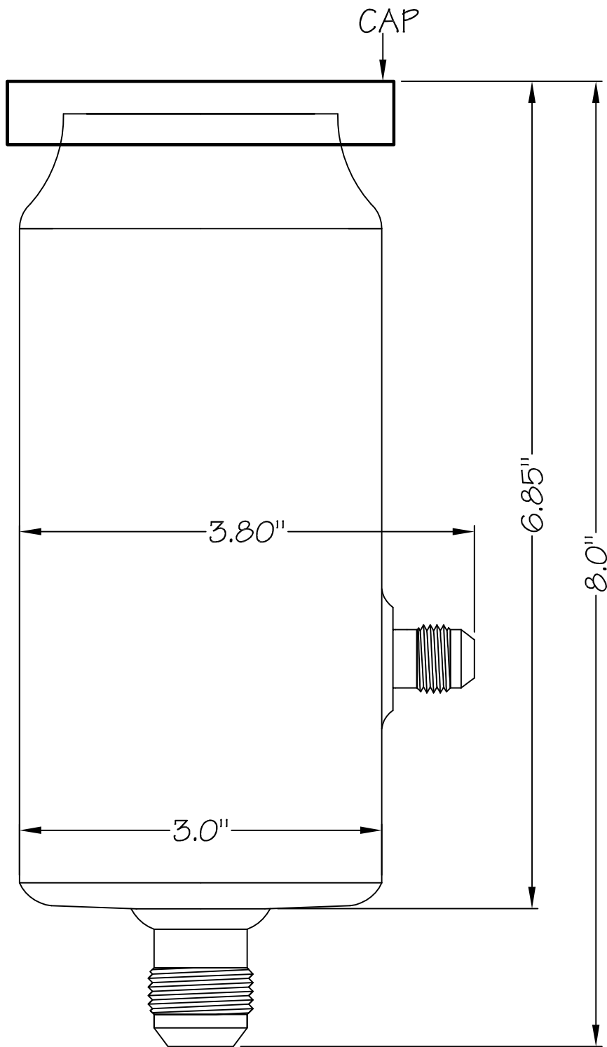
KRC Round Economy & Deluxe Reservoir Tank
