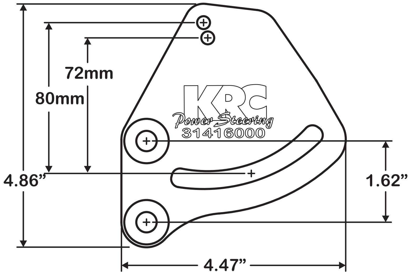
Small Block Chevrolet Left Block
