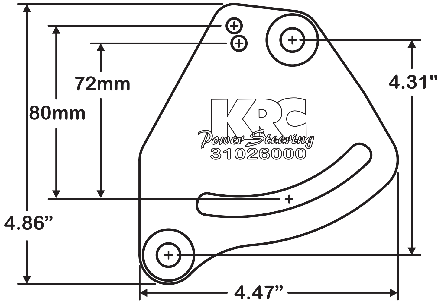
Big Block Chevrolet Left Block
