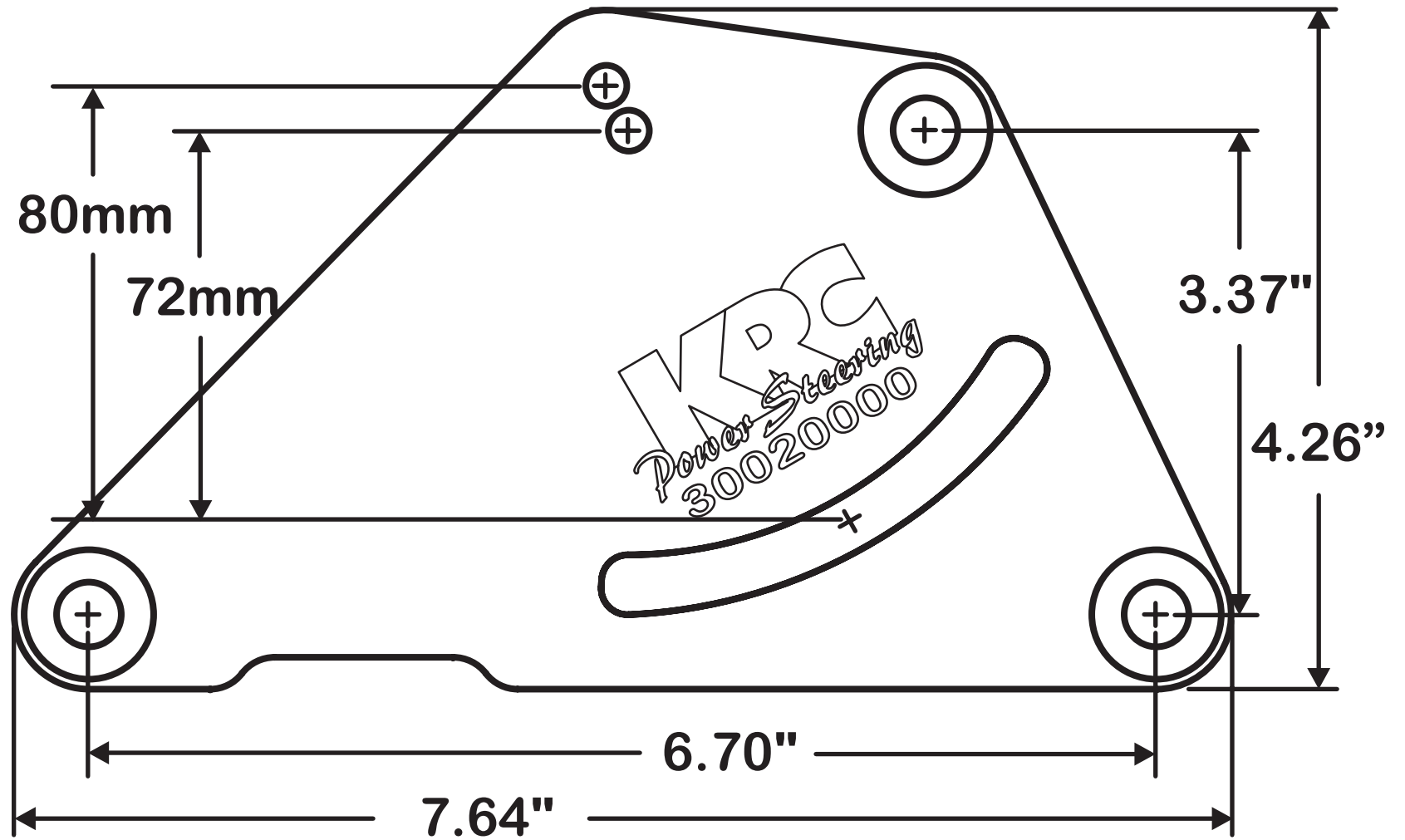
Big Block Chevrolet Left Head
